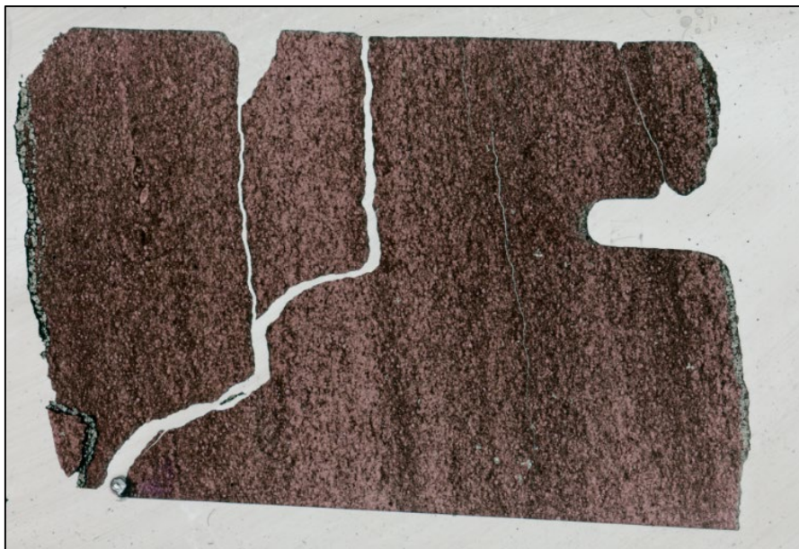
Figure: Thin section photograph of a sample of Marcellus Shale from Harrison County, West Virginia. Depth of sample is 7,206 feet. Thin section is ~2 inches long and ~one inch high.
