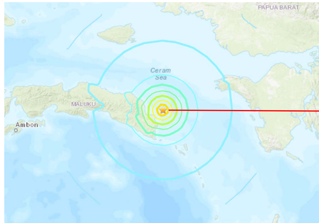
USGS Community Internet Intensity Map SERAM, INDONESIA
